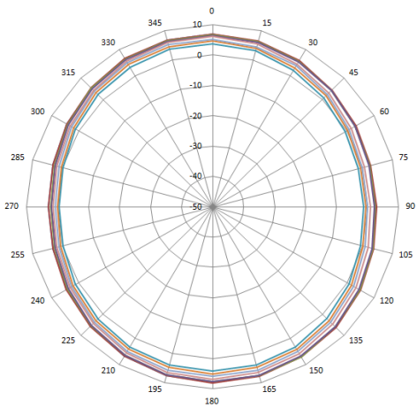
5GHz-H Plane
