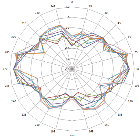
5GHz-E Plane
