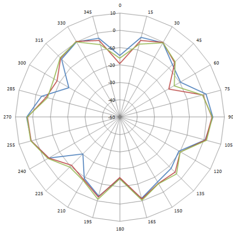
2.4GHz-E Plane
