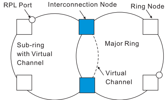
Figure 271: Sub-ring with Virtual Channel
