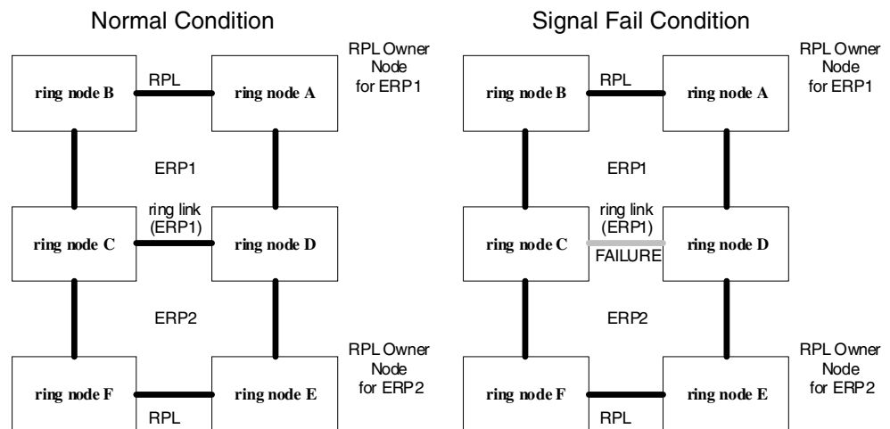
Figure 269: Ring Interconnection Architecture (Multi-ring/Ladder Network)
