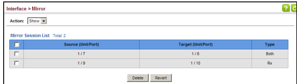
Figure 62: Displaying Local Port Mirror Sessions
