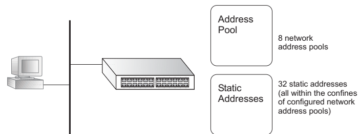
Figure 472: DHCP Server
