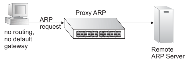
Figure 416: Proxy ARP
