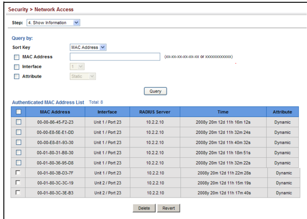
Figure 185: Showing Addresses Authenticated for Network Access
