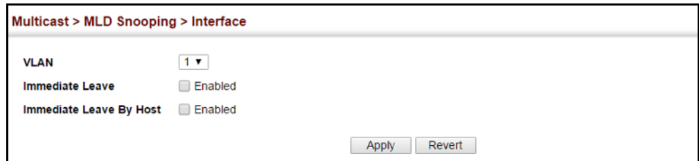
Figure 365: Configuring Immediate Leave for MLD Snooping
