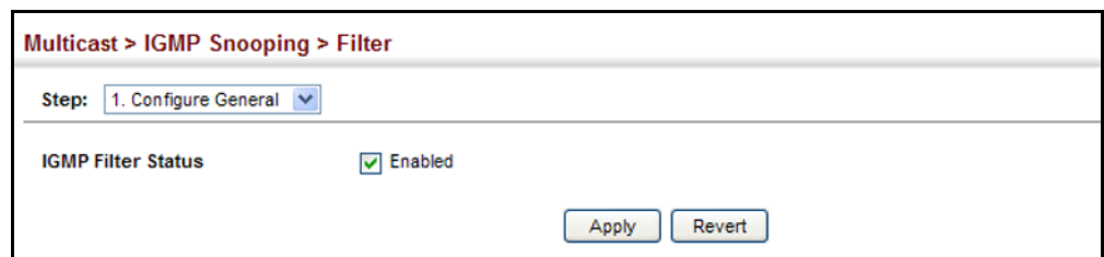
Figure 358: Enabling IGMP Filtering and Throttling
