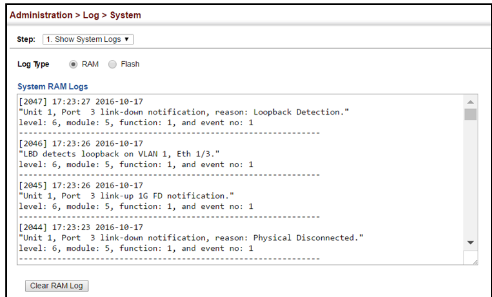
Figure 237: Showing Error Messages Logged to System Memory
