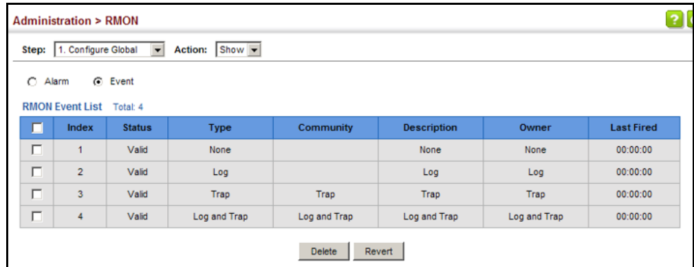
Figure 281: Showing Configured RMON Events
