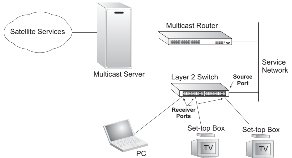
Figure 386: MVR Concept
