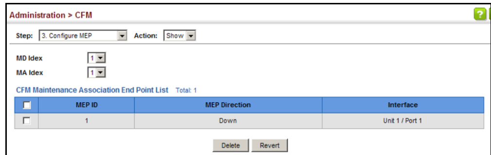
Figure 318: Showing Maintenance End Points
