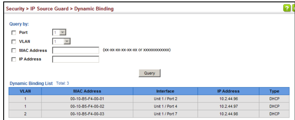
Figure 225: Showing the IPv4 Source Guard Binding Table
