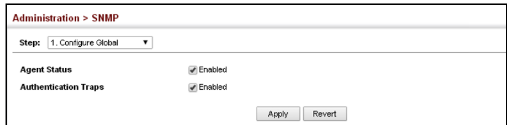
Figure 254: Configuring Global Settings for SNMP
