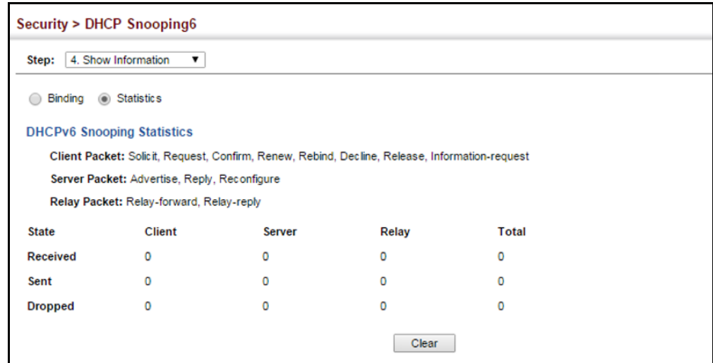
Figure 221: Displaying Statistics for DHCPv6 Snooping
