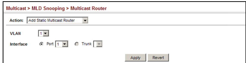
Figure 366: Configuring a Static Interface for an IPv6 Multicast Router
