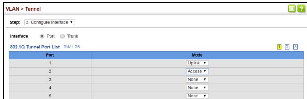
Figure 90: Adding an Interface to a QinQ Tunnel
