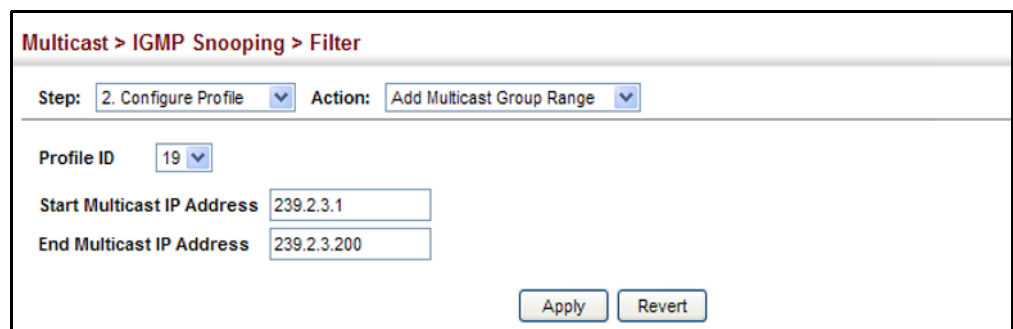
Figure 361: Adding Multicast Groups to an IGMP Filtering Profile
