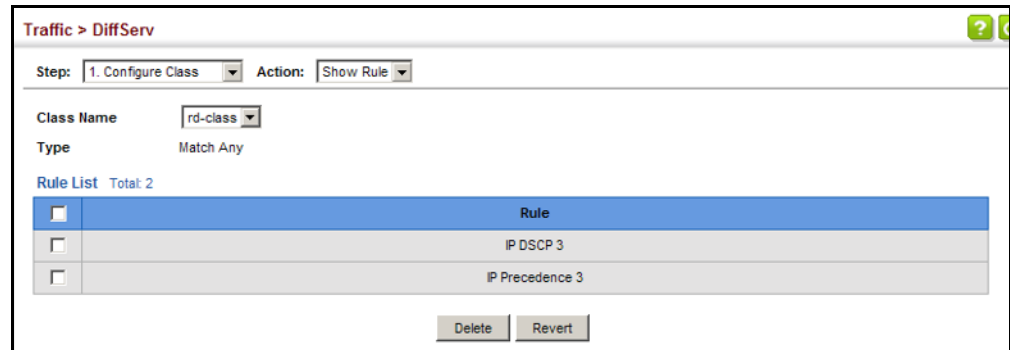
Figure 148: Showing the Rules for a Class Map
