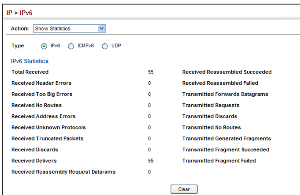
Figure 431: Showing IPv6 Statistics (IPv6)
