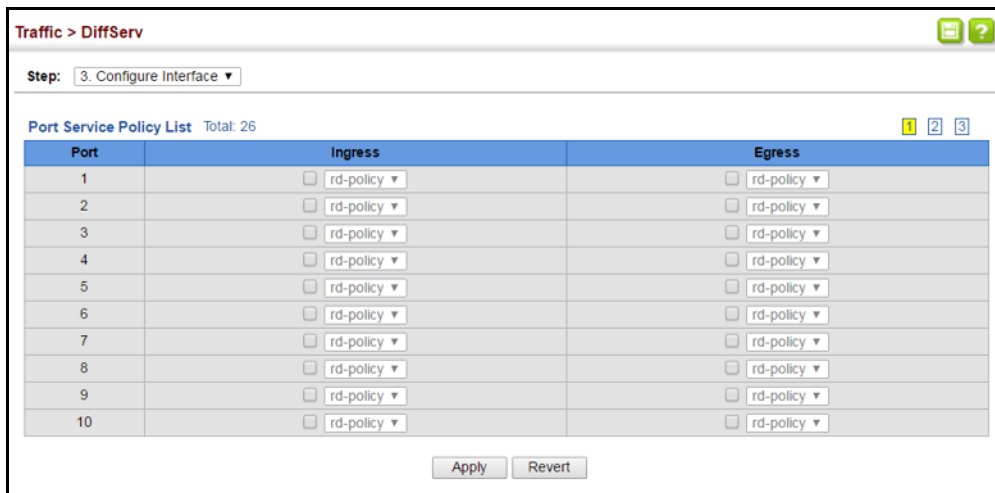
Figure 153: Attaching a Policy Map to a Port
