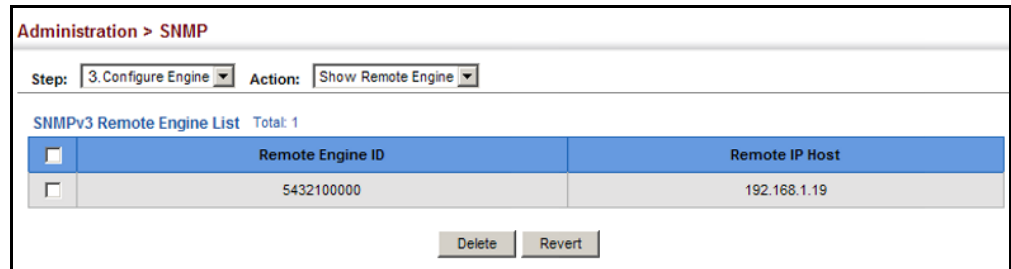
Figure 259: Showing Remote Engine IDs for SNMP
