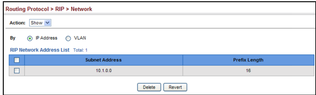
Figure 443: Showing Network Interfaces Using RIP
