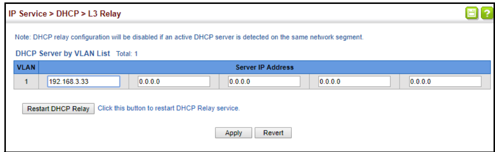
Figure 468: Configuring L3 DHCP Relay Service
