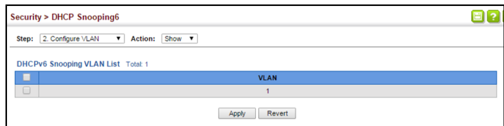
Figure 218: Showing VLANs Enabled for DHCPv6 Snooping
