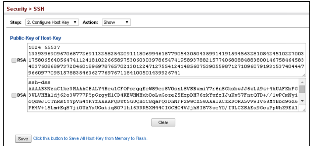
Figure 190: Showing the SSH Host Key Pair
