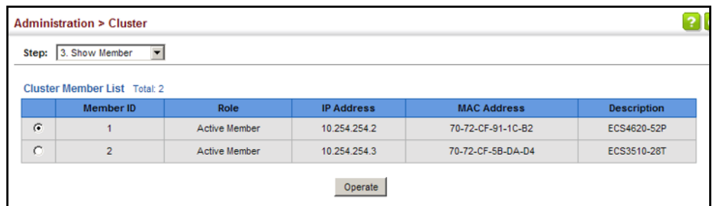
Figure 292: Managing a Cluster Member
