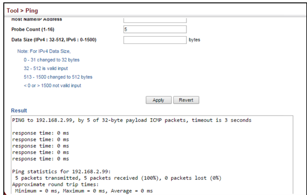
Figure 414: Pinging a Network Device
