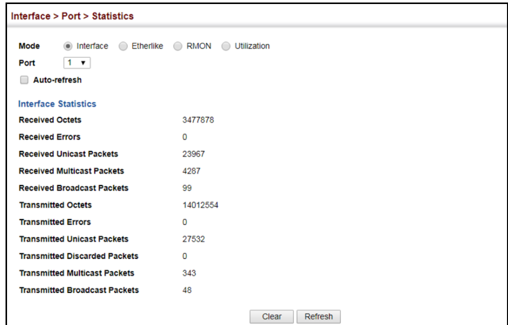
Figure 33: Showing Port Statistics (Table)
