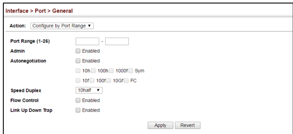
Figure 31: Configuring Connections by Port Range
