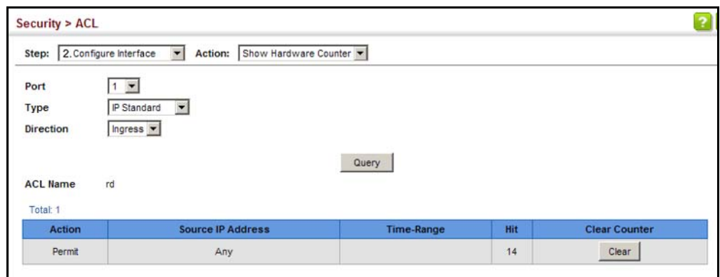
Figure 203: Showing ACL Statistics
