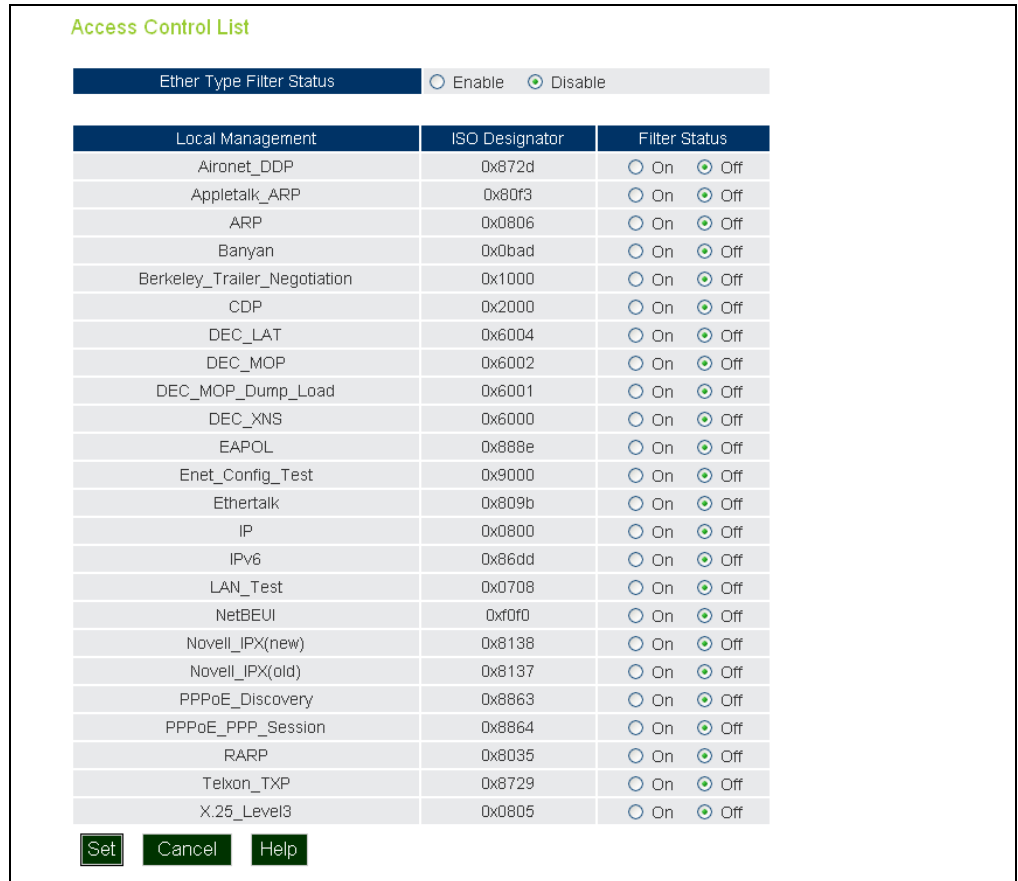
Figure 24: Ethernet Type Filter
